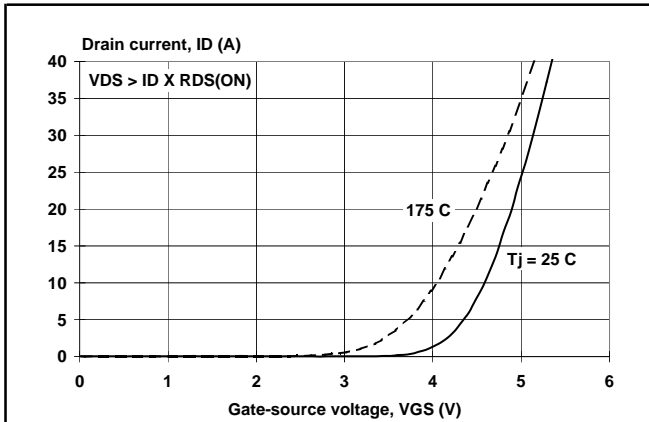
Fig. 7. Typical transfer characteristics.
