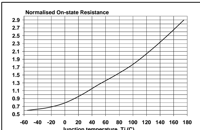
Fig. 9. Normalised drain-source on-state resistance.
