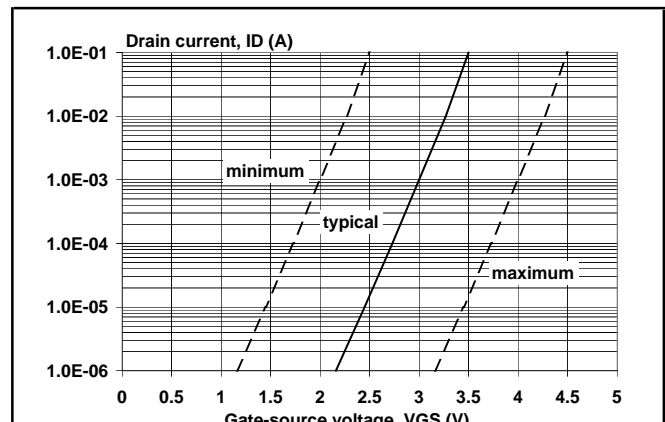
Fig. 11. Sub-threshold drain current.
