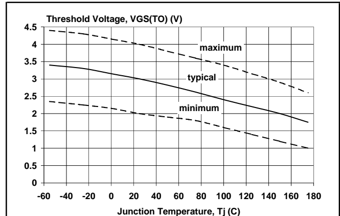
Fig. 10. Gate threshold voltage.
